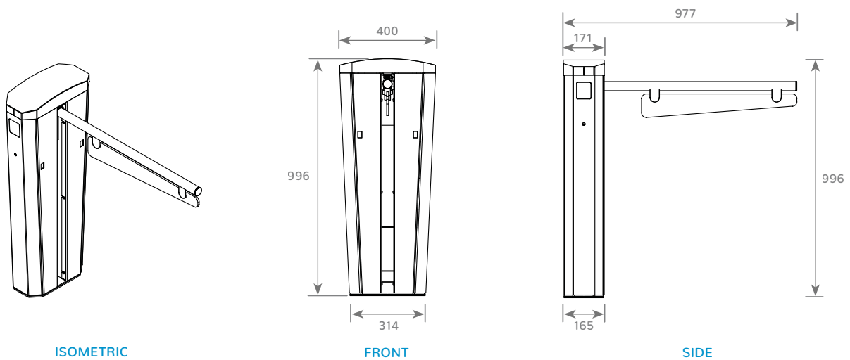
ISOMETRIC
