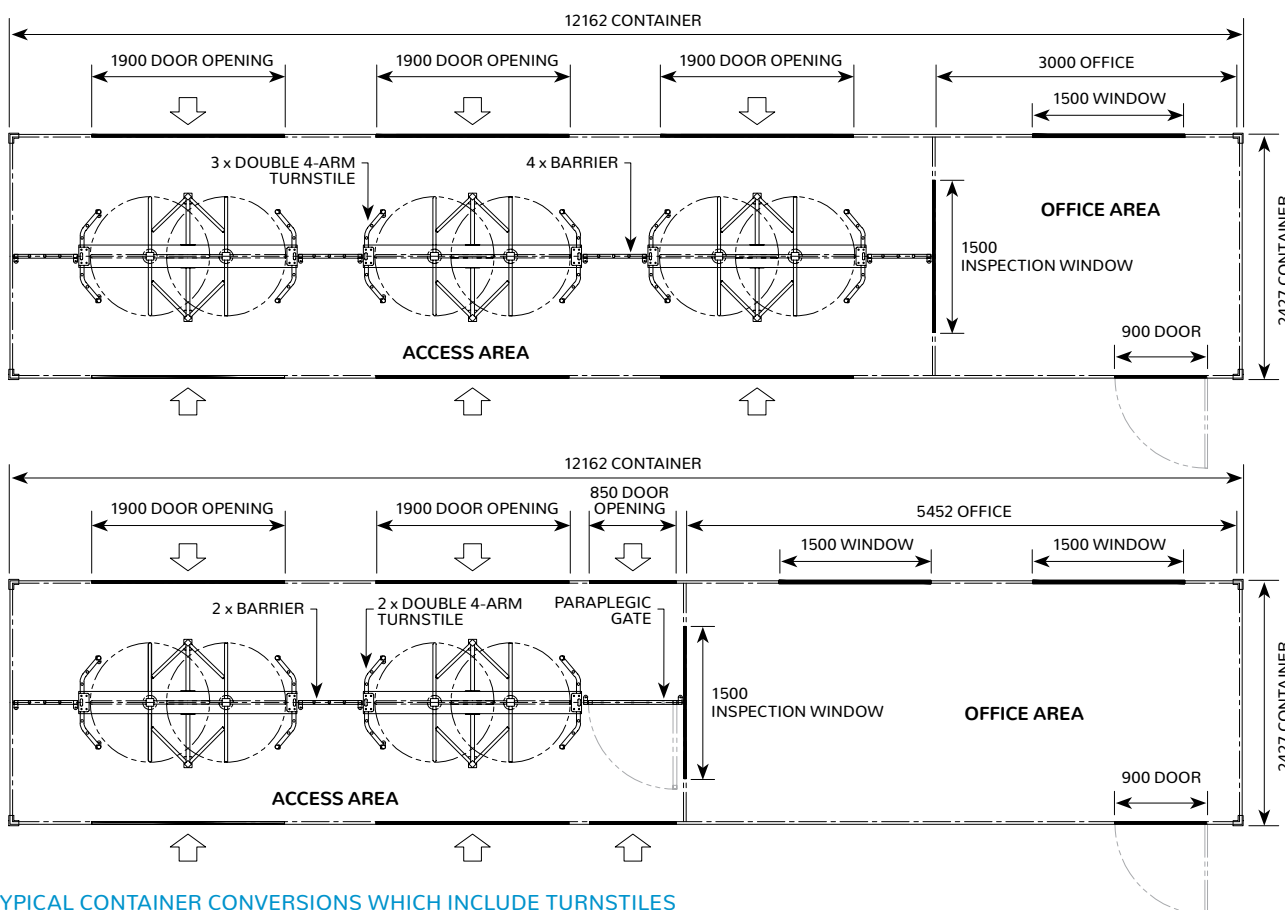
TYPICAL CONTAINER CONVERSIONS WHICH INCLUDE TURNSTILES
